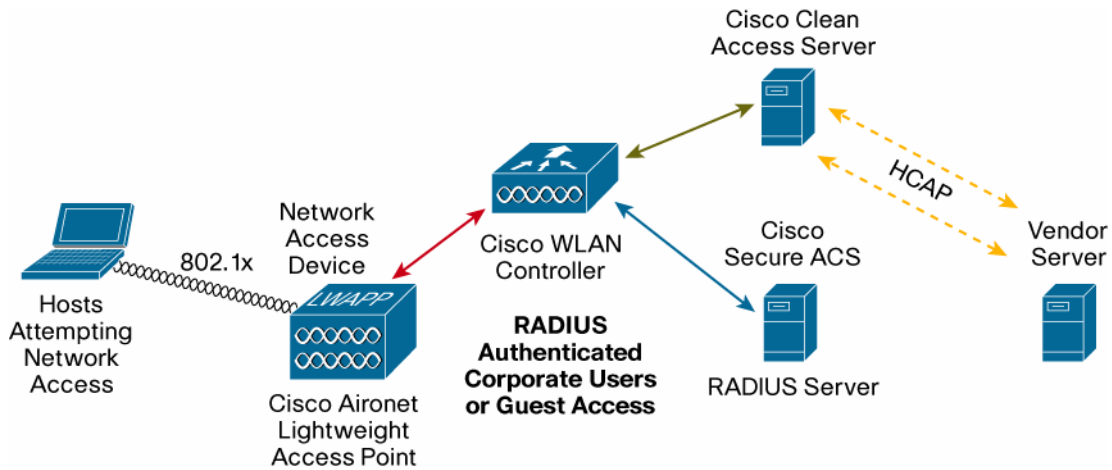
Figure 4. NAC Framework Architecture for Cisco Unified Wireless Network
